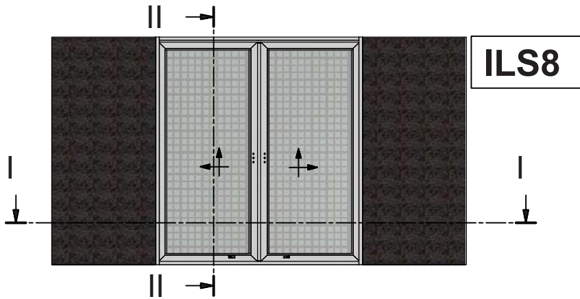
Two Sash Meeting Stile Pocket Lift & Slide Window with Flyscreen and Shutter Short sash use only S560
