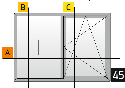
Single side-hung casement, tilt and turn, with fixed hidden sash
