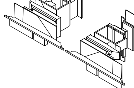
End cap for sash inversion profile S67758
