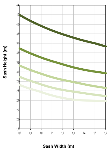
Maximum Panel Dimensions For Given Wind Pressure Class A ... L/150 deflection limit
