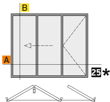
OUTWARD OPENING, 2+1 3-PANELS FOLDING DOOR LOW THRESHOLD
