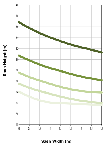
Maximum Panel Dimensions For Given Wind Pressure Class A ... L/150 deflection limit
